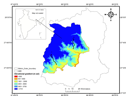
Fig 1 Location of study sites in the Khangchendzonga Biosphere Reserve (1 depicts Yuksom-Black Kabru transect and 2 depicts Tholung- Kisong transect)
