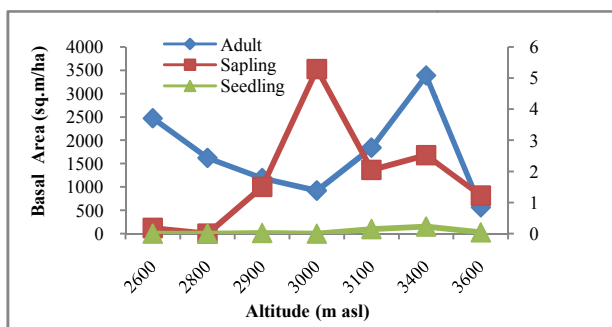
Fig 4 Basal area of woody species of the habitat of the Satyr Tragopan in the Khangchendzonga Biosphere Reserve
