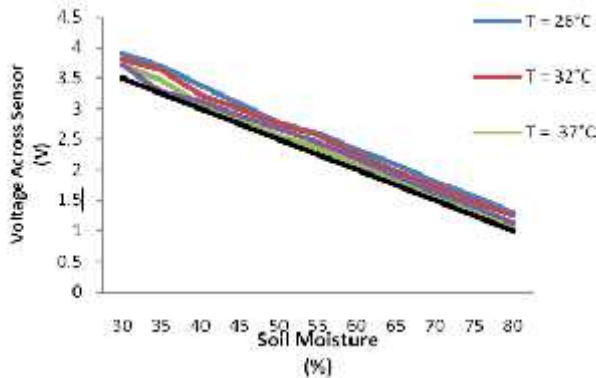
Fig.4 Variation in soil moisture at different temperature
