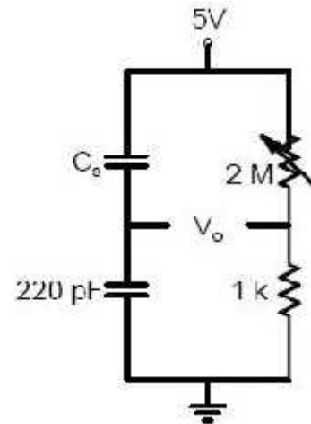
Fig.3 Moisture sensor
