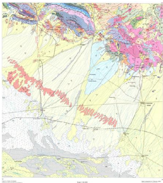
Fig1 Geology of area
