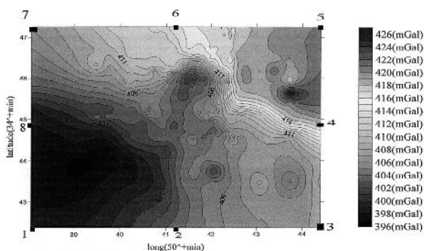
Figure 2 complete bouguer anomaly with density (2.1)g/cm 3
