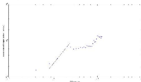
Figure 3 Complete regression line of bouguer anomaly of the area with optimal density (2/5g/cm^3) with fractal dimension (2.24)
