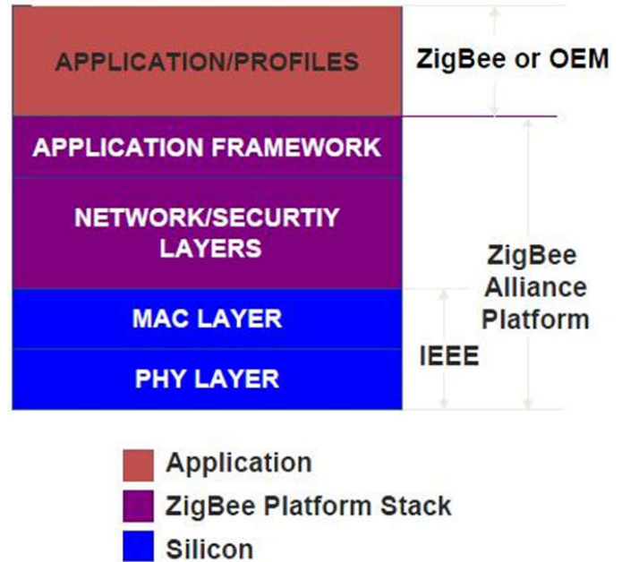
Fig 2 IEEE802.15.4/ZigBee protocol stack architecture
